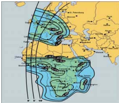
SATIP4 KU Footprints W3A (yellow), IS10 (blue)
